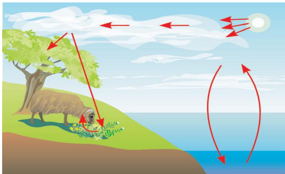
Figure 7.5: 14 C is formed in the upper atmosphere. Cosmic rays produce neutrons which collide with 14 N nuclei ( ^{14}\text{N} + \text{n} \rightarrow ^{14}\text{C} + \text{p} ).
