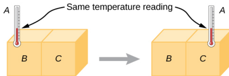
Figure 4.1: If thermometer A is in thermal equilibrium with object B, and B is in thermal equilibrium with C, then A is in thermal equilibrium with C. Therefore, the reading on A stays the same when A is moved over to make contact with C.
